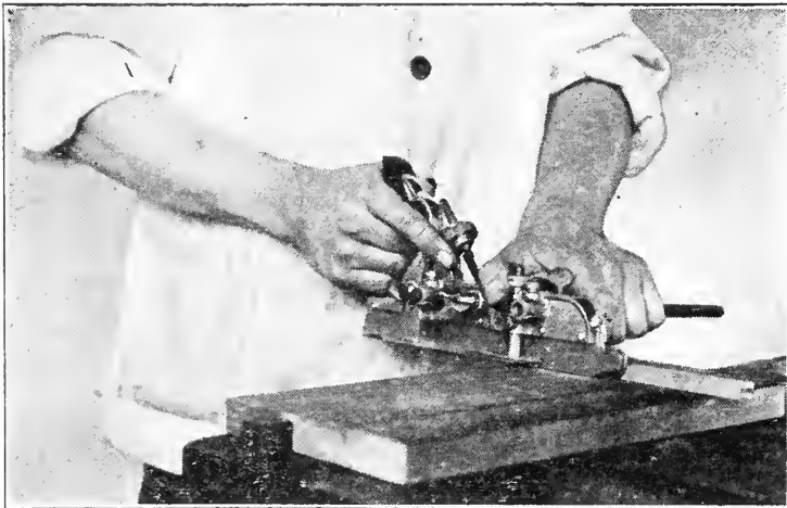
FIG. 71. PLANING DADO JOINT.
